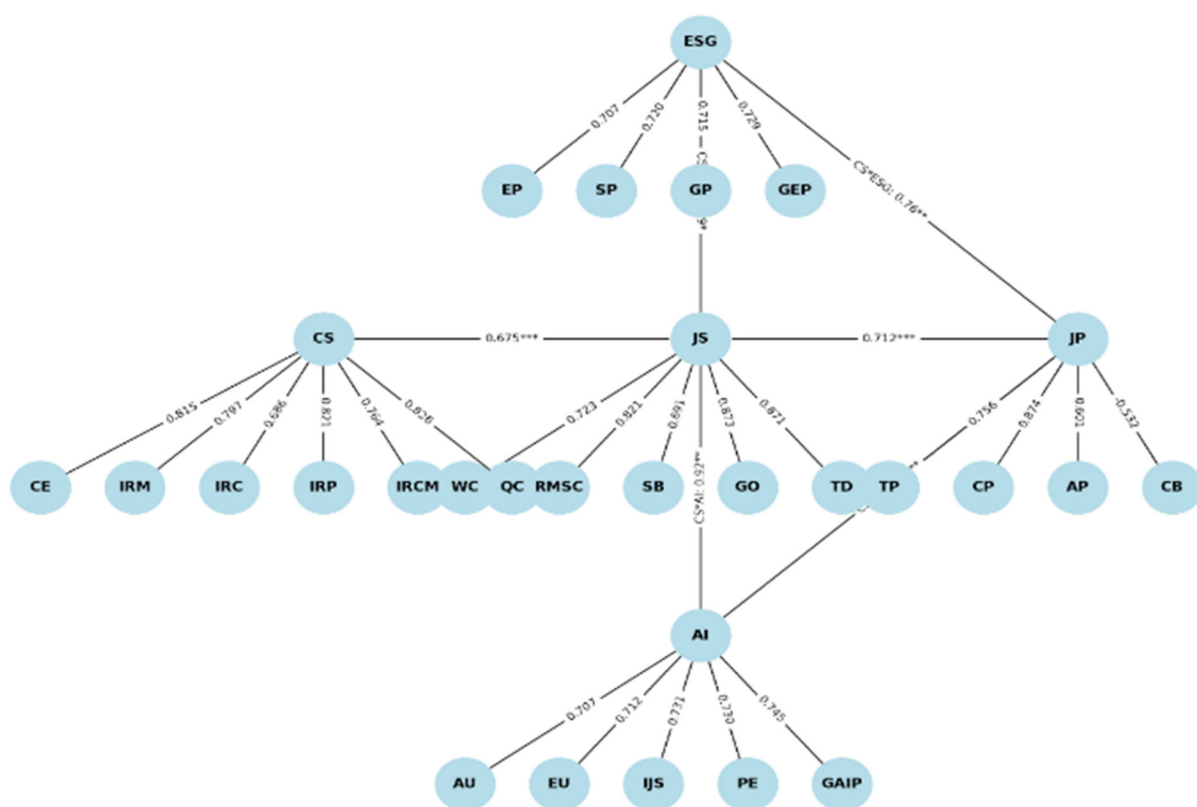
Figure 2. Path Analysis
